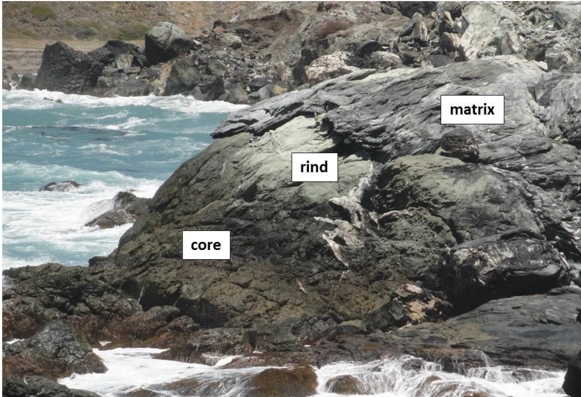
Figure 10: Lawsonite-blueschist core, rind, and matrix in Crab Cove, Santa Catalina Island. The mélangé matrix concentrically wraps around the rind and block core.
