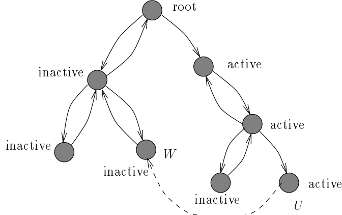
FIG. 3. Contracted graph G'/S .
