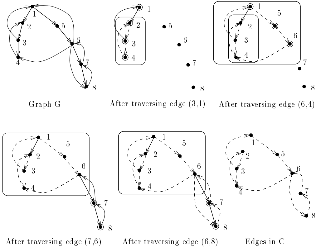
FIG. 6. Example to illustrate execution of algorithm.
