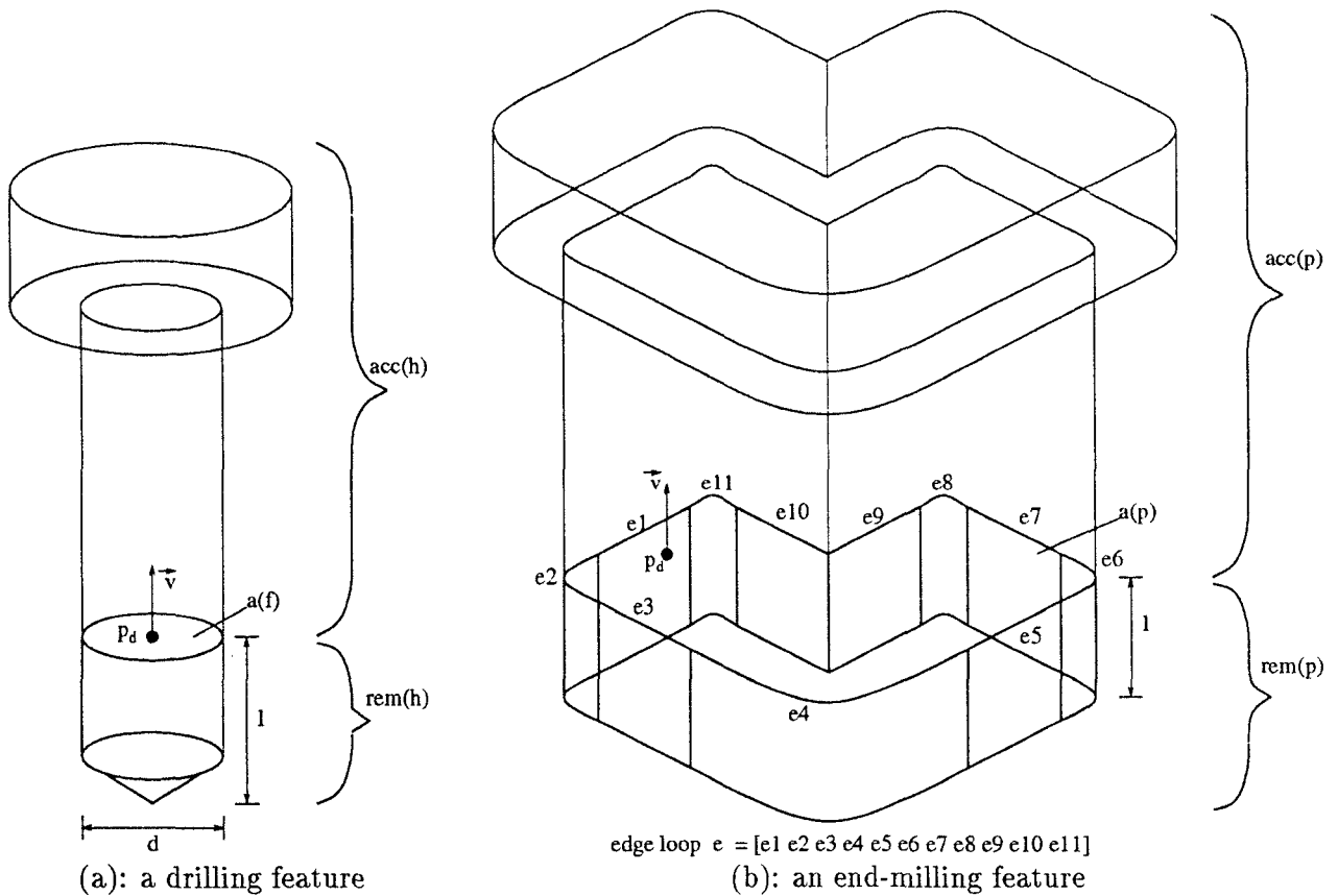
Figure 3: Examples of machining features.
