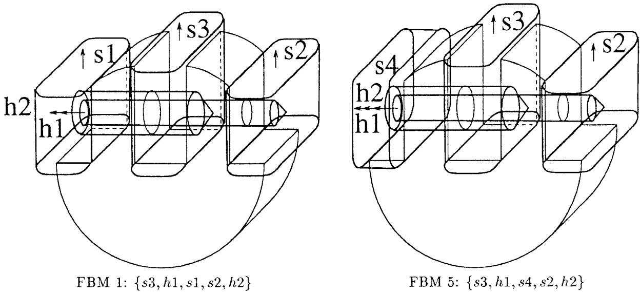
Figure 14: The two primary FBMs generated by our algorithm.
