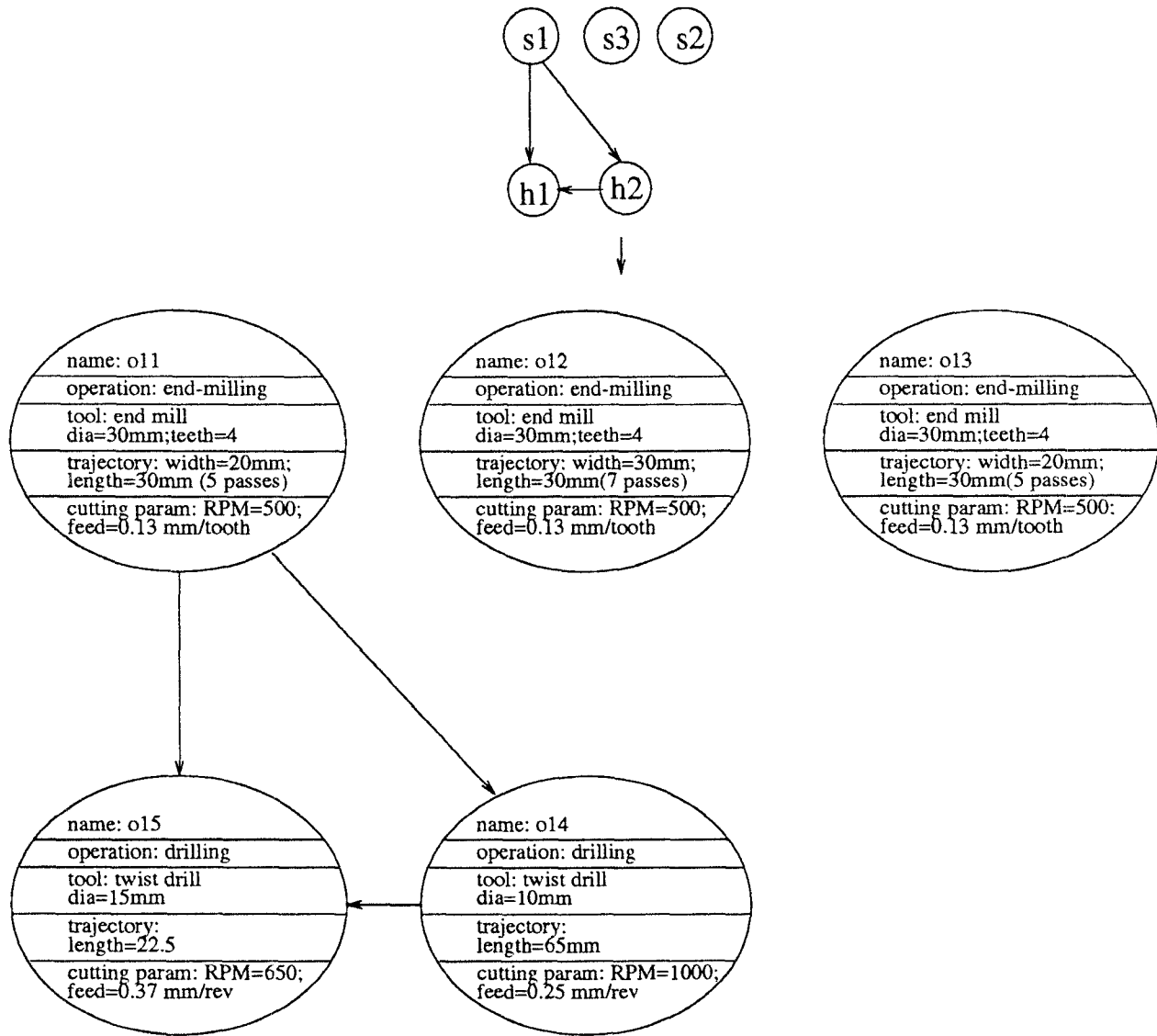
Figure 19: Details of Operation Plan OP1 for Design 1.
