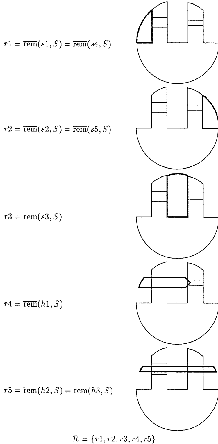
Figure 12: Effective removal volumes of features in \mathcal{F} , where \mathcal{F} is as shown in Fig. 11.
