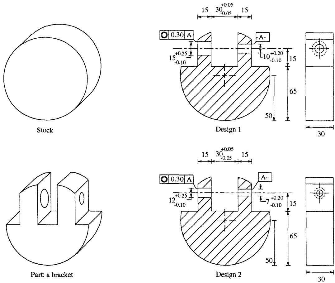
Figure 9: Two possible designs for a bracket.
