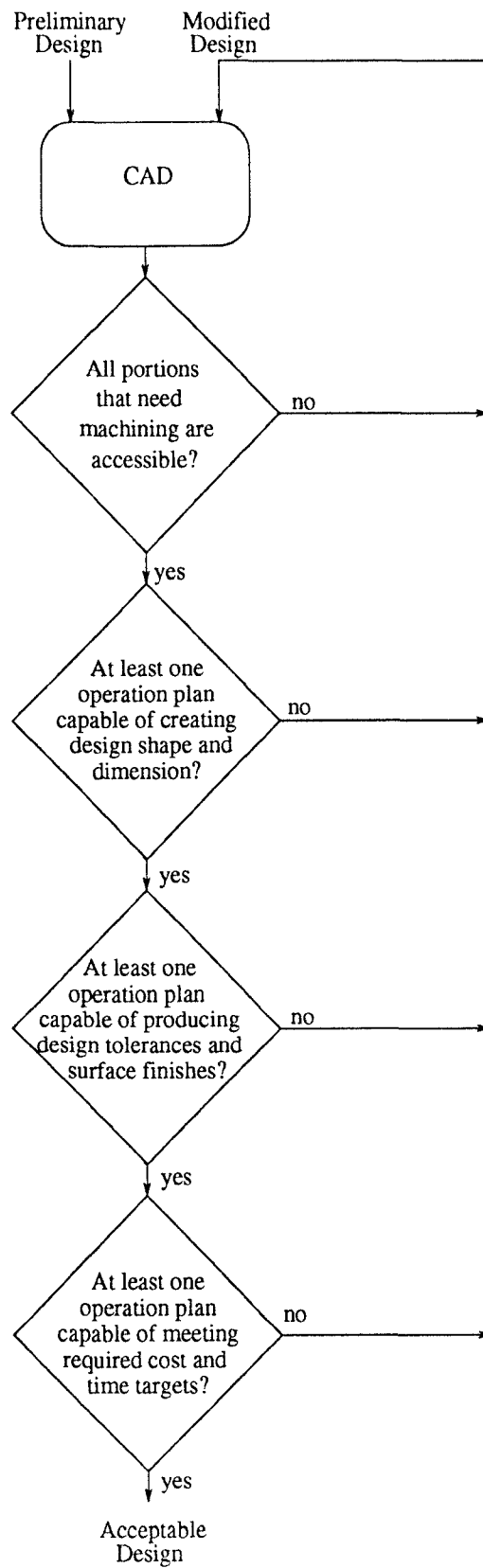
Figure 2: Manufacturability analysis.
