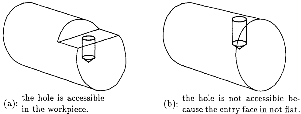
Figure 5: Examples of feature accessibility.
