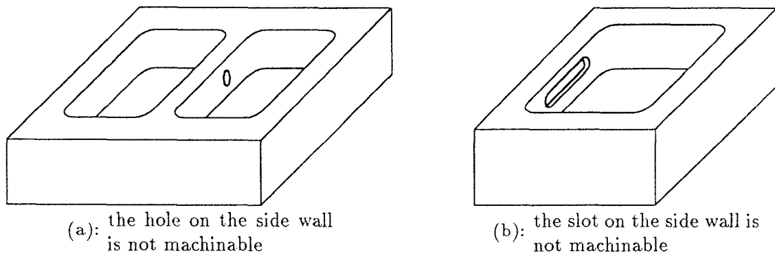
Figure 8: Examples of unmachinable parts, when the set of available machining operations \mathcal{M} is {drilling, end-milling}.
