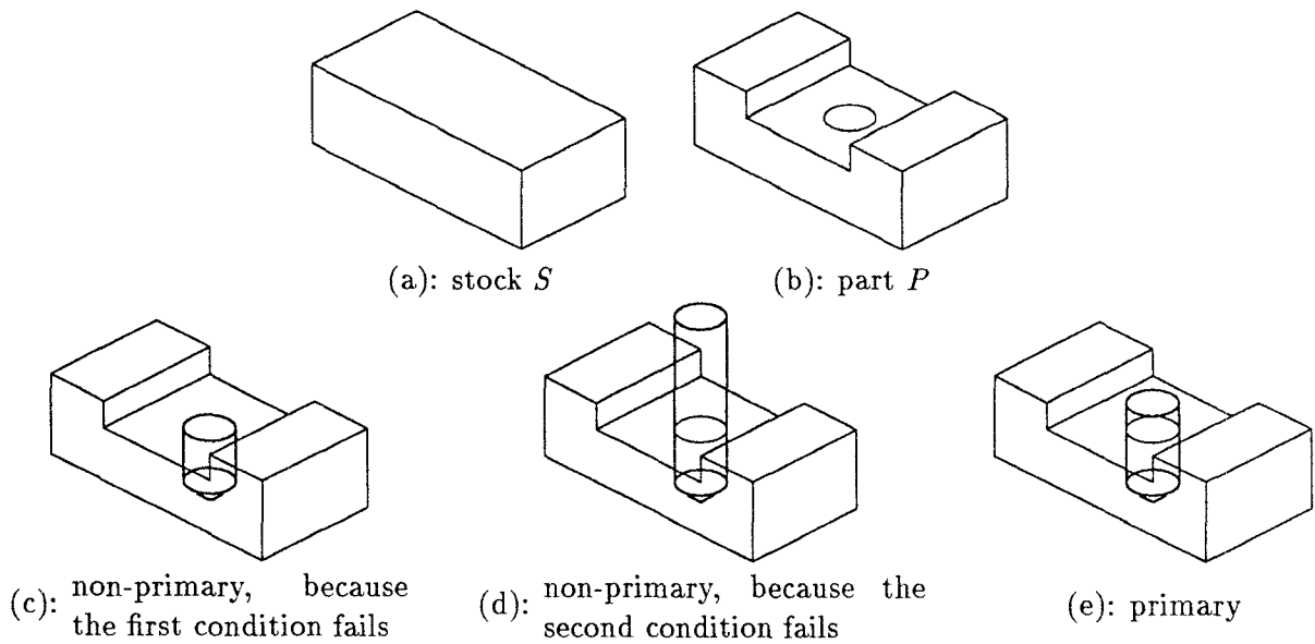
Figure 7: Example of primary and non-primary features.
