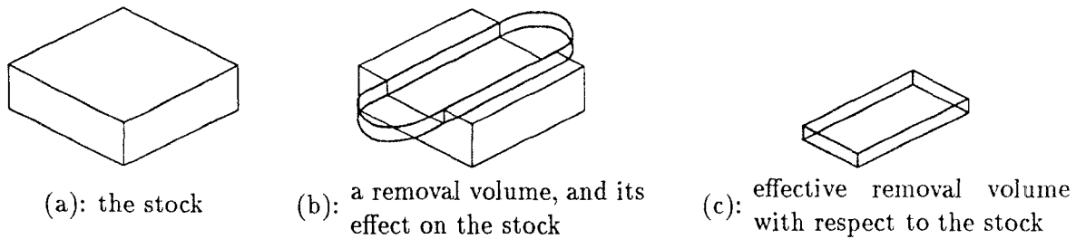
Figure 4: An end-milling feature and its effective removal volume.
