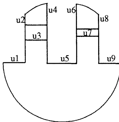
Figure 10: Faces to be created for Design 1. For Design 2, the faces are similar, except that they have different dimensions.
