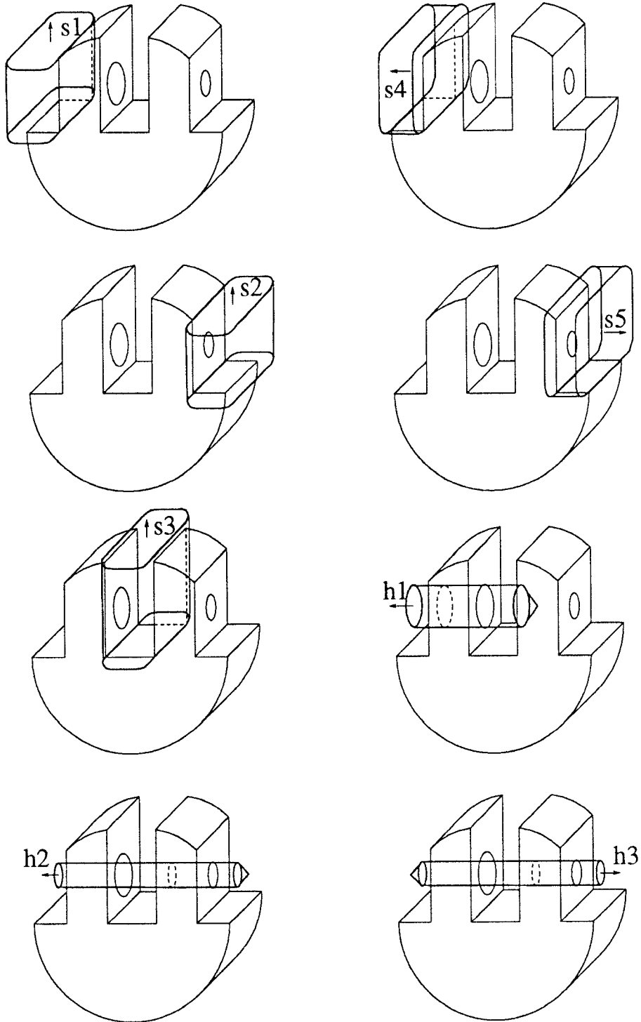
Figure 11: Features identified by our algorithm for Design 1 of Fig. 9. For Design 2, the features are identical, except that the holes have different diameters.
