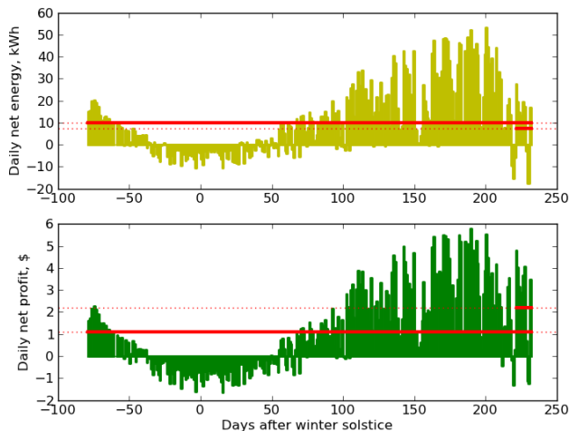
Figure 4. Top: daily net energy production for reACT virtual located in College Park, MD; daily net profit associated with selling excess power is shown as the green bottom plot. Mean and most-recent 10-day mean values are illustrated by the red horizontal bars.
