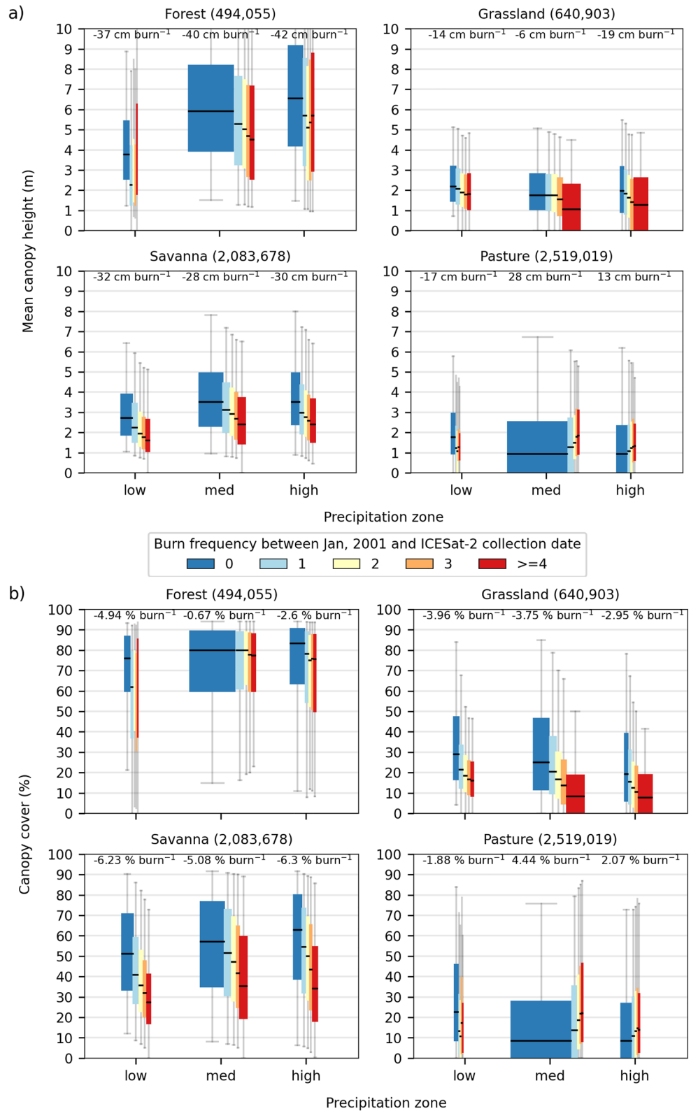
Figure 3. (a) Mean canopy heights (in m) and (b) canopy cover (%) decreased with increasing burn frequency for all natural cover types across all precipitation zones. Figures in brackets represent the number of 20-m segments over each land cover type. The width of each individual box plot is proportional to the number of segments available for a given land cover type and precipitation zone. Numbers at the top of each subplot represent the slope of the line of best fit through the medians of the boxplots for the burn frequency classes 0, 1, 2, and 3 for each precipitation zone.
