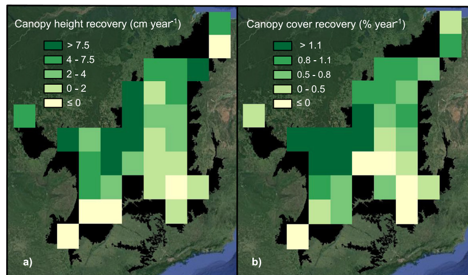
Figure 5. Spatial maps of (a) canopy height and (b) canopy cover recovery for Savannas at 2° resolution shows a clear east-west gradient, with higher recovery values in areas receiving more rainfall. For each 2° pixel, 20-m segments over the savanna were grouped into four time-since-burn classes—0–5, 5–10, 10–15, and 15–20 years. Canopy height recovery for each 2° pixel was defined as the slope of the line fitted through the median canopy height for each time-since-fire class. Recovery values were calculated for only those 2° pixels, which have at least 100 segments in each time-since-burn class.
