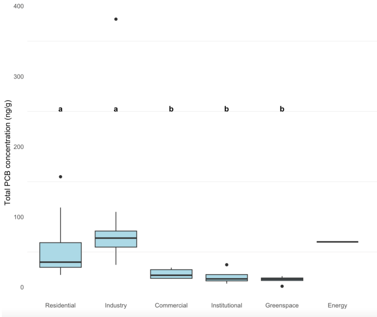
Figure 3.3. Total PCB concentrations across different land use types.
