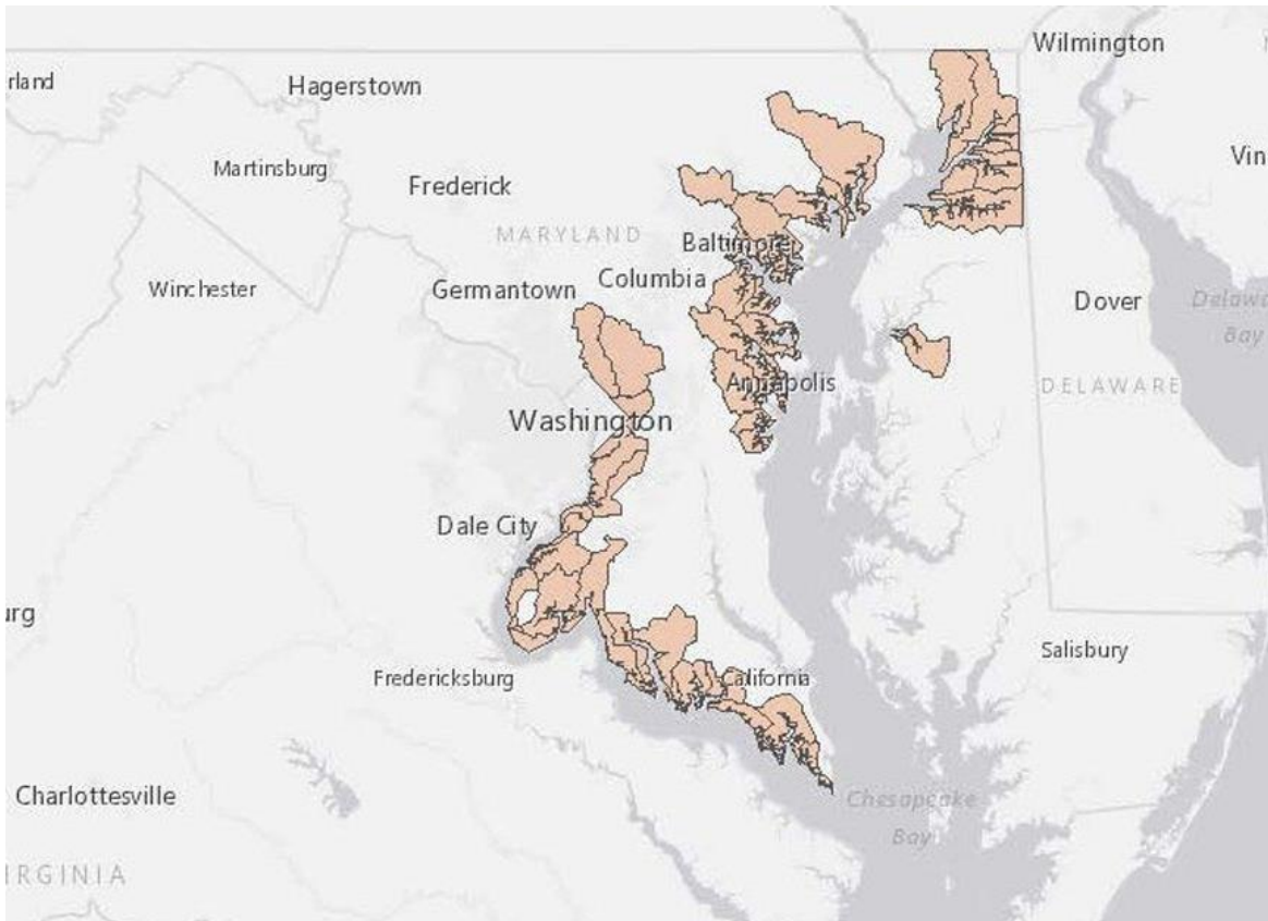
Figure 1.2. Map of PCB TMDL watersheds in Maryland.
