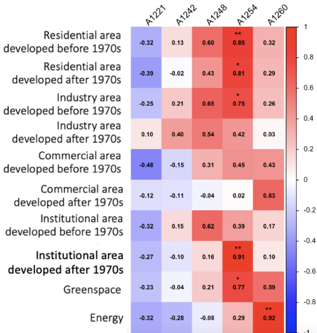
Figure 3.8. Spearman correlation coefficients between homologue distribution of soil and stormwater sediment from different categories and Aroclors after remove mono- and di PCBs.
