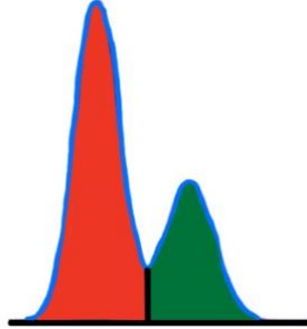
Figure B.1. Drop method for determining the areas under overlapping peaks.
