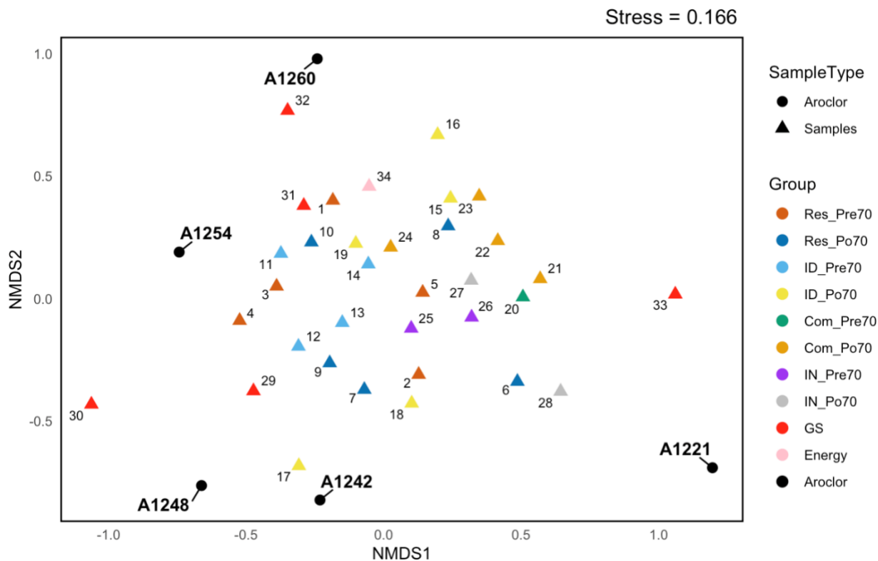
Figure 3.7. NMDS plot of each sample and Aroclor mixtures.
