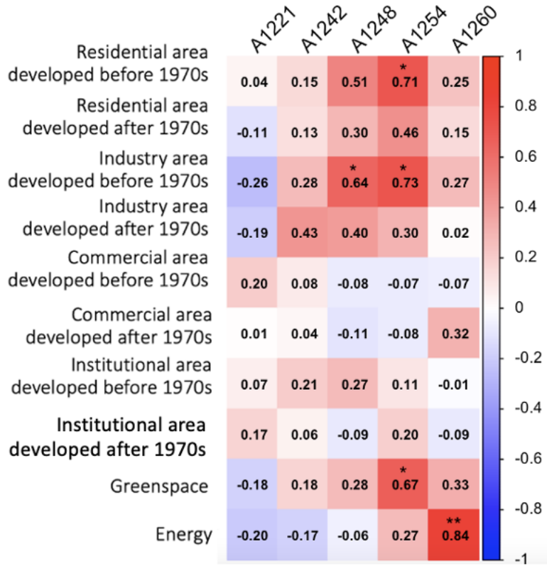
Figure 3.6. Spearman correlation coefficients between homologue distribution of soil and stormwater sediment from different categories and Aroclors.
