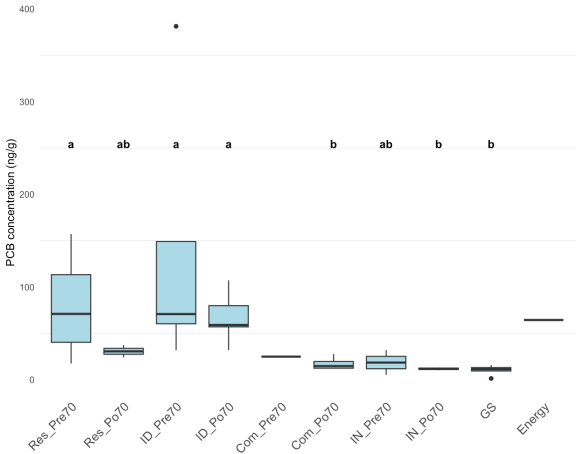
Figure 3.5. Comparison of total PCB concentrations across land use types developed before and after 1970s.
