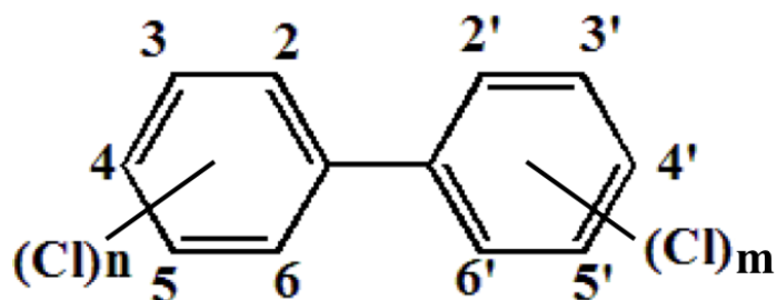
Figure 1.1. Structure of PCBs
