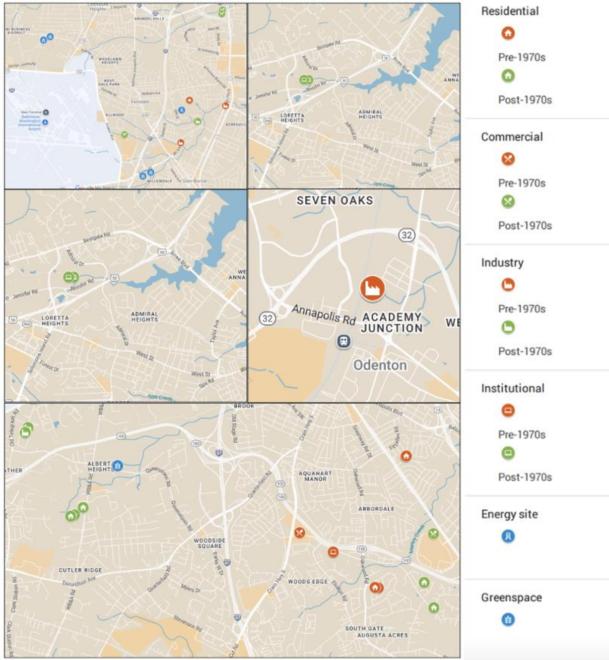
Figure 2.2. Map of the sampling sites.
