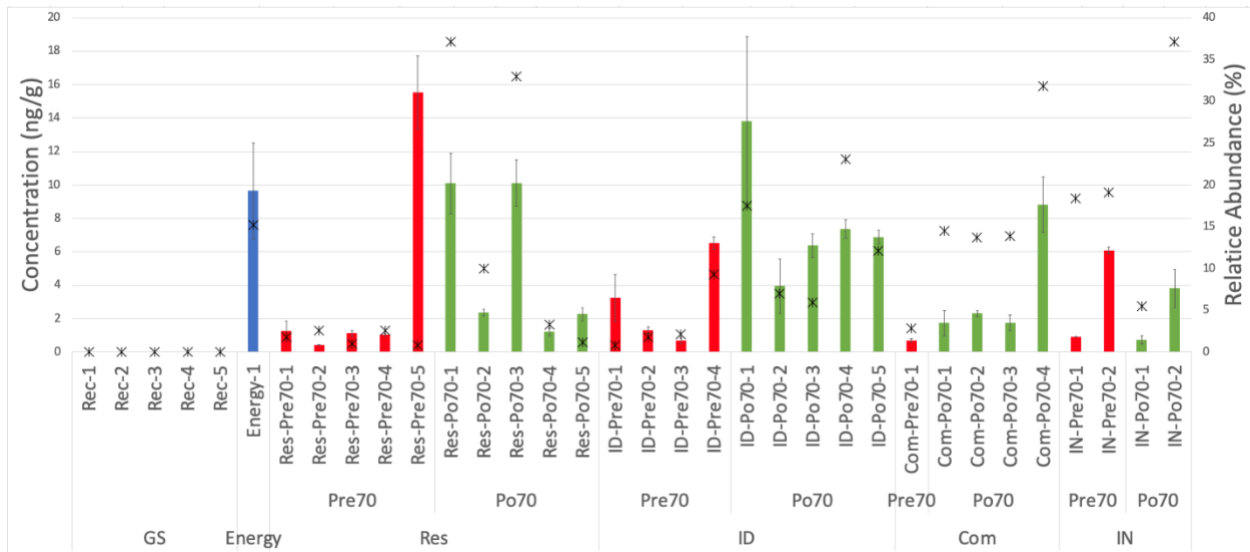
Figure 3.10. PCB 11 concentration (bar (left axis)) and mass relative abundance (x (right axis)).
