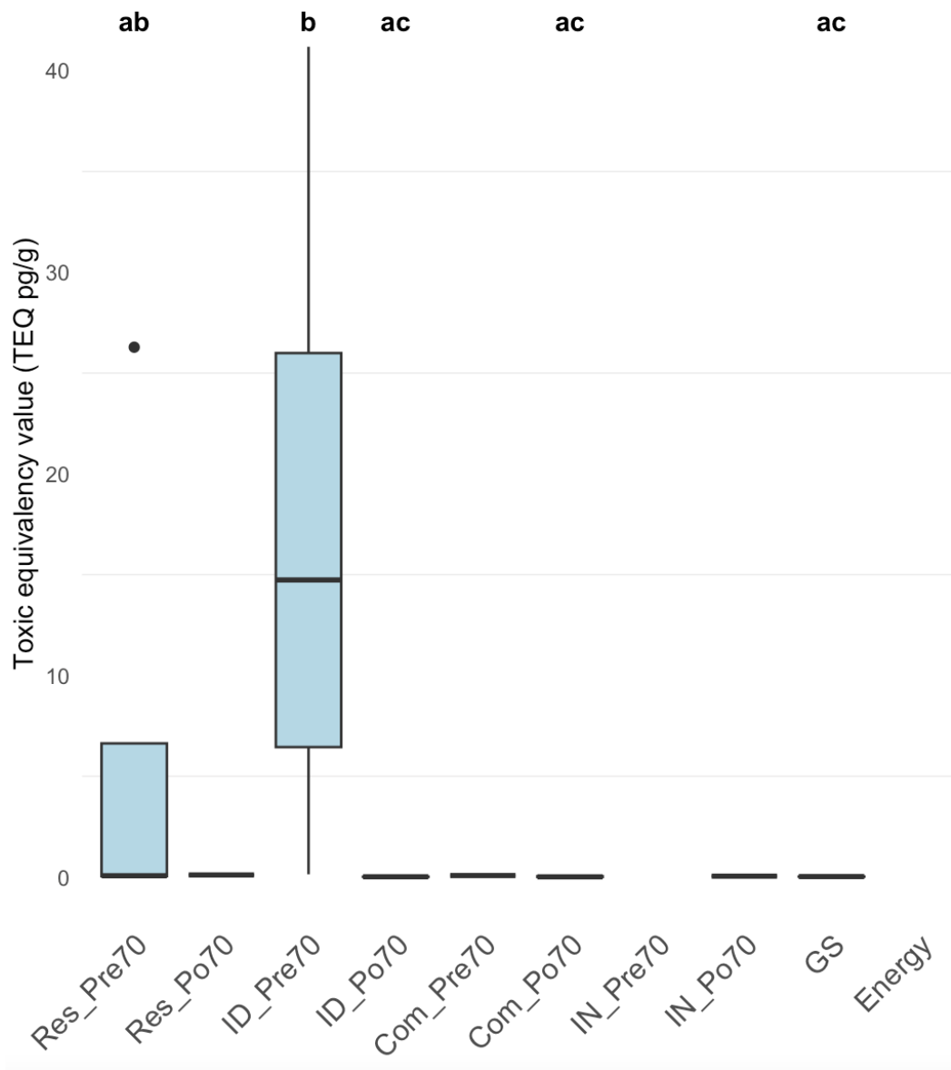
Figure 3.11. Comparison of toxic equivalency value across land use types developed before and after 1970s.
