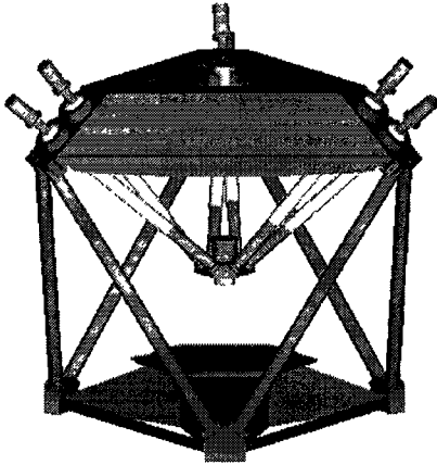
FIGURE 1. NIST INGERSOLL OCTAHEDRAL-HEXAPOD
