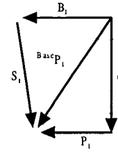
FIGURE 5. INVERSE KINEMATIC VECTORS
