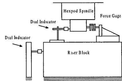
FIGURE 6. EXPERIMENTAL SET-UP FOR Z = 1268 MM
