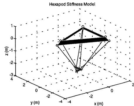
FIGURE 2A. MACHINE POSITION (-0.3 M, 0.3 M, 0.3 M) MACHINE ORIENTATION (-30, 0, 0) (DEGREES)
